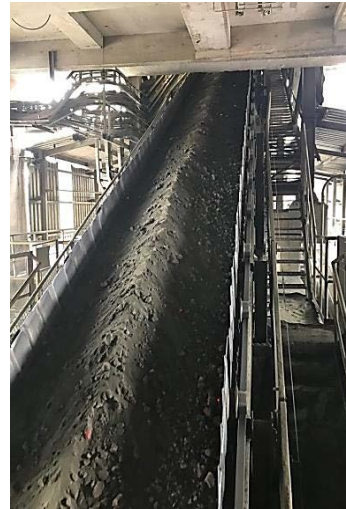
Deep Pan Conveyor feeding Cement Mill Hopper
